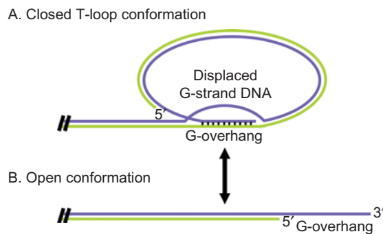
Figure 1. Telomere cycling between (A) closed and (B) open conformations.
